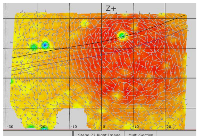
Fig. 11. Analysis of the displacement of black dots on the surface of the specimen at the end of the test
