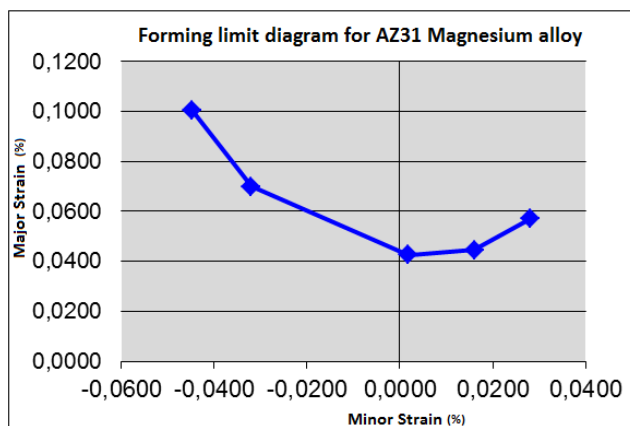
Fig. 13. Forming limit diagram built through the average values of the minor and major strains
